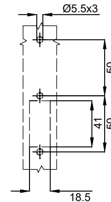
开孔尺寸 (Cut Out)
