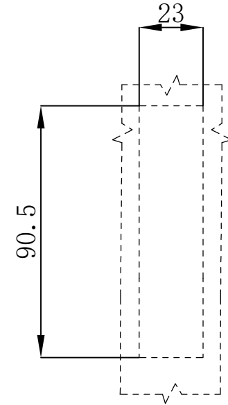
开孔尺寸 (Cut Out)
