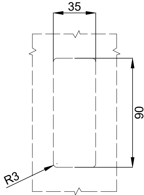
开孔尺寸 (Cut Out)
