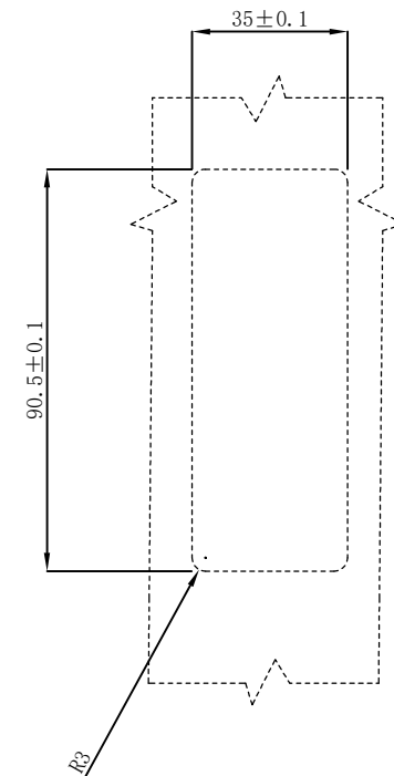
开孔尺寸 (Cut Out)
