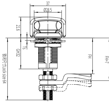
可调节款 Adjustable compression height
