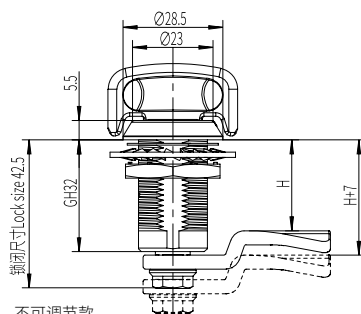
不可调节款 Non-adjustable compression height
