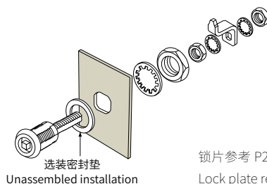
选装密封垫 Unassembled installation
